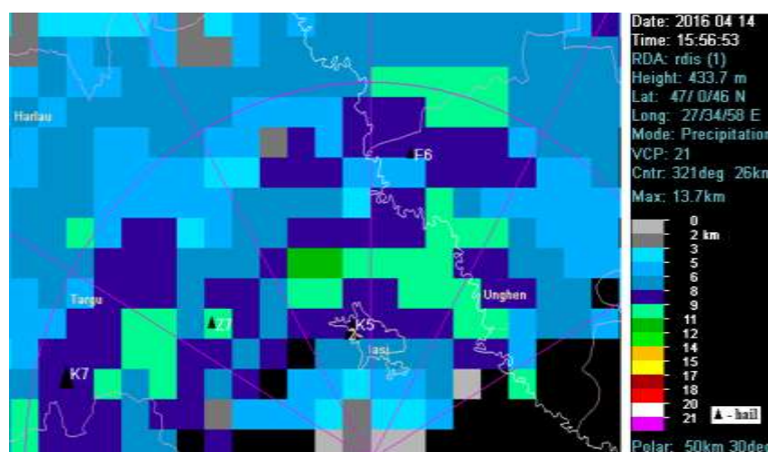
Fig. 11. Locations with hail and height of clouds estimated by Doppler radar from Bârnova, Iași county
