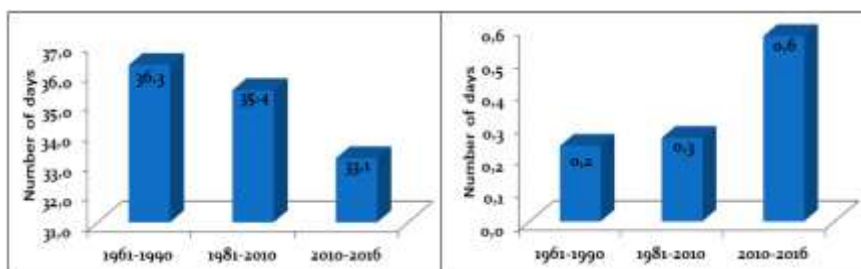
Fig. 5. Periodically number of days with precipitation \geq 0.1 mm and \geq 30 mm per day in the spring season at Iași meteorological station from the periods of 1961 – 1990, 1981 – 2010 and 2010-2016
