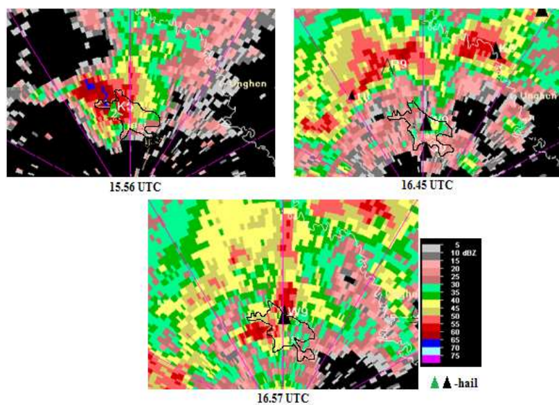
Fig. 12. Radar reflectivity and locations where have occurred hail
