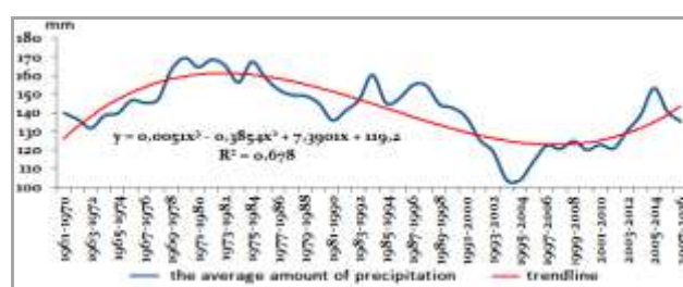
Fig. 2. The moving averages over a 10-year time series, shifted successively with one year of the average precipitation amounts in the spring at Iași meteorological station (1961 – 2016)
