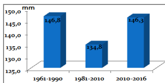
Fig. 3. Periodically mean amounts of the atmospheric precipitation quantities in the spring at Iași meteorological station from the periods of 1961 – 1990, 1981 – 2010 and 2010-2016
