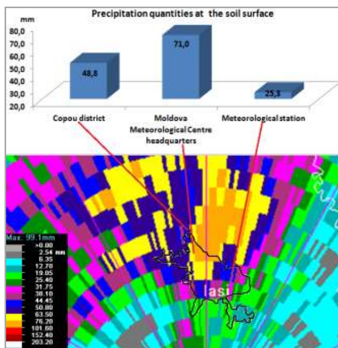
Fig. 14. Precipitation quantities - estimation during 24 hour (13.04.2016, 20.00 UTC – 14.04.2016, 20.00 UTC) with Doppler radar and precipitation data measured at soil surface
