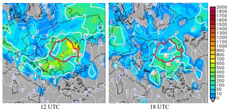
Fig. 10. Lifted Index (K) mixed layer Convective Available Potential Energy (CAPE) on 14 April 2016, 12 and 18 UTC (source: www.wetter3.de )
