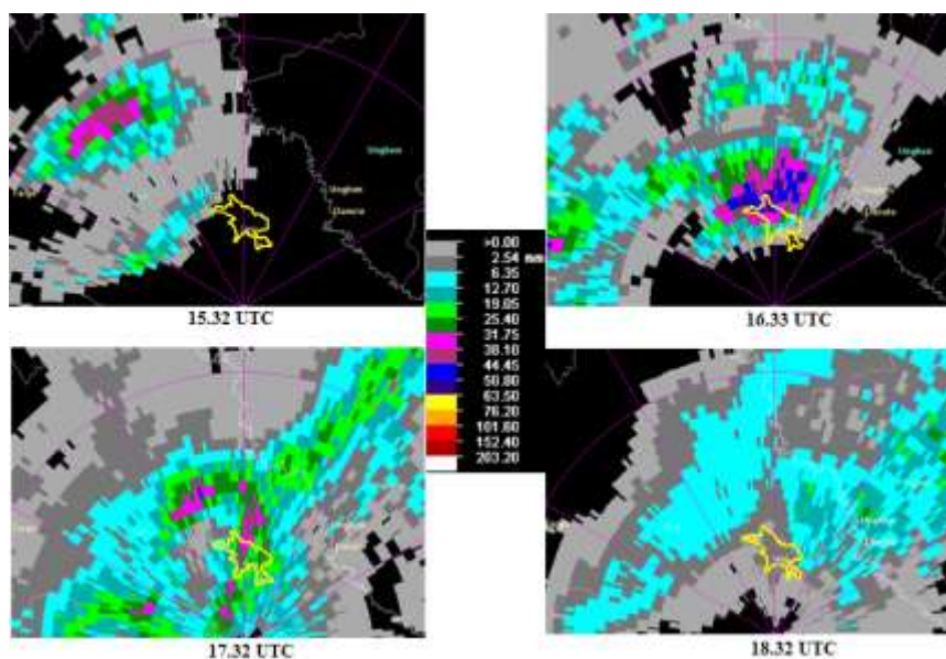
Fig. 13. Estimation of precipitation quantities during 1 hour with Doppler radar located at Bârnova, Iași county
