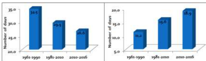
Fig. 4. Periodically number of days with rain and number of shower days in the spring season at Iași meteorological station from the periods of 1961 – 1990, 1981 – 2010 and 2010-2016
