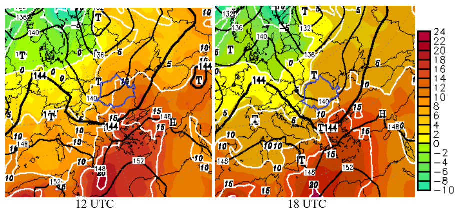
Fig. 9. The geopotential (gpdam) and surface-level air isobaric temperature (°C) of 850 hPa on April, 2016 at 12 and 18 UTC (source: www.wetter3.de )
