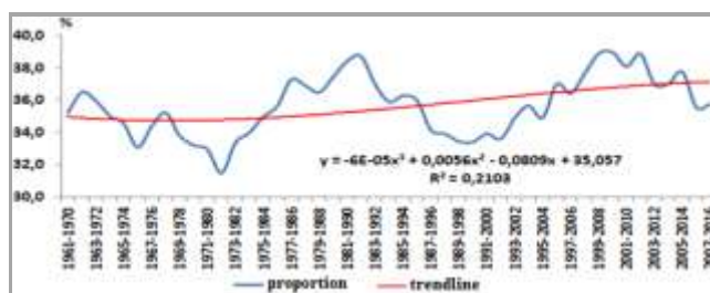
Fig. 6. The evolution of the proportion of maximum quantities of rainfall in 24 hours from the total monthly quantities in the spring seasons at Iași meteorological station
