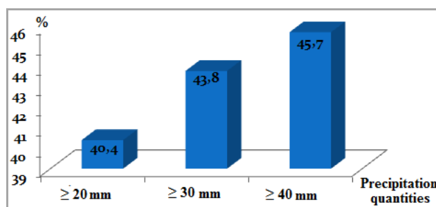
Fig. 7. The mean proportion of maximum quantities of rainfall in 24 hours (on various thresholds) from the total monthly quantities in the spring seasons at Iași meteorological station (1961-2016)
