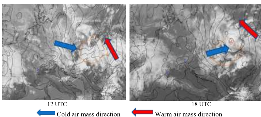
Fig. 8. Synoptic situation on 14 April 2016, 12 and 18 UTC at ground level (source: http://eumetrain.org/eport.html )
